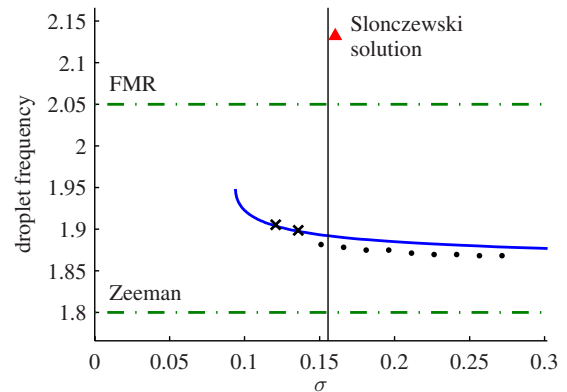
FIG. 7. (Color online) Dots: perturbed droplet frequency as a function of current with the Oersted field computed from micromagnetic simulations. Crosses: perturbed droplets that undergo a drift instability; the frequency is calculated before the instability manifests. Solid curve: droplet frequency as a function of the sustaining current from Eq. (20). Dashed-dotted: the Zeeman ( h_0 ) and FMR ( h_0+h_k-1 ) frequencies. Triangle: the Slonczewski critical current and onset frequency for high-symmetry (Ref. 8) (see Appendix A). Solid vertical line: numerically computed threshold current in the presence of the Oersted field and the canted fixed layer. Parameter values are the same as in Fig. 6.
